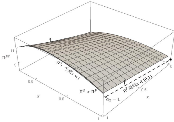
图 6 (b) \delta 足够小的情况 ( \rho = 0.28, H = 0.98, L = 0.01, p = 13.14, c = 4, \delta = 1.01 )
